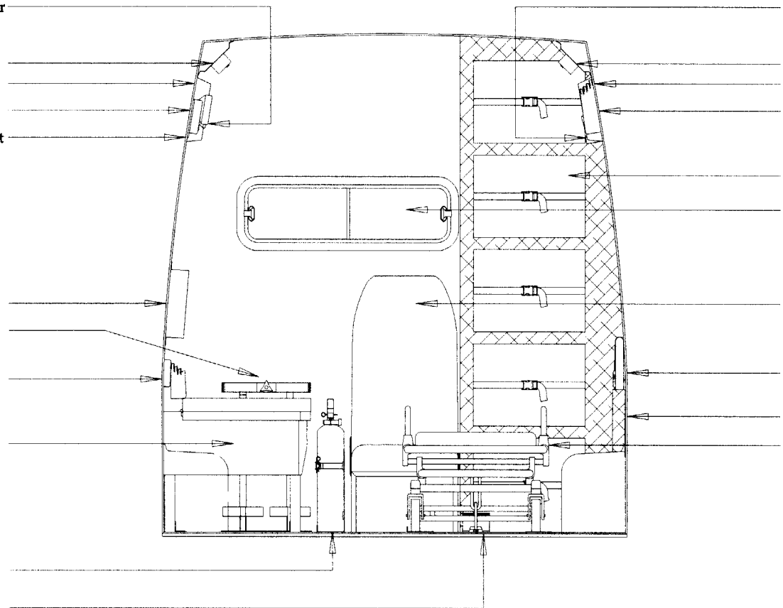
Back Elevation
