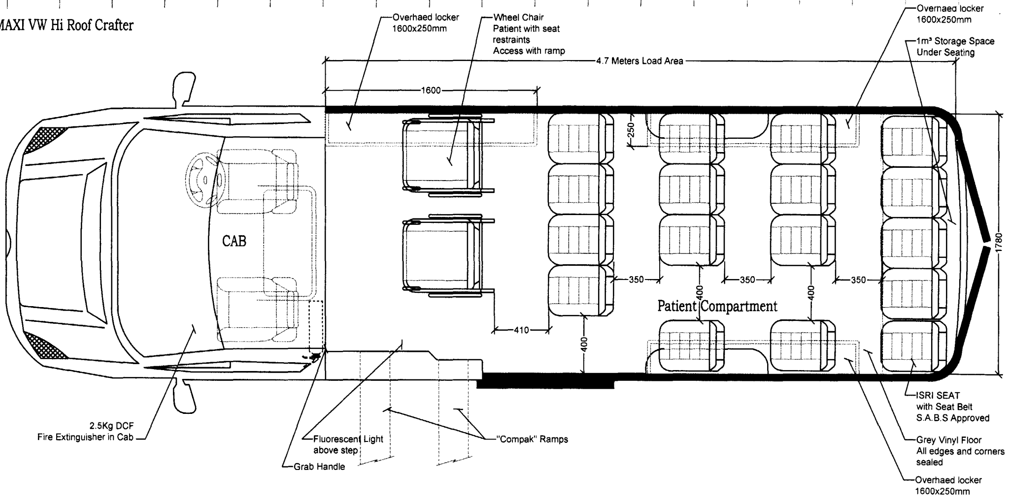
Plan View
