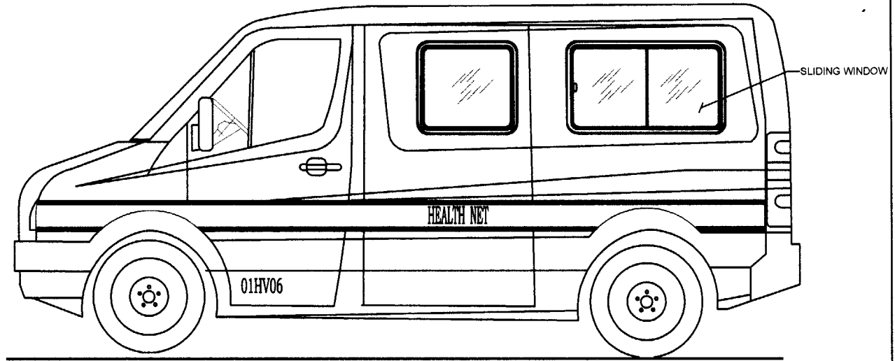
LHS ELEVATION
