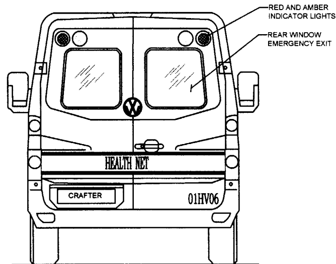
REAR VIEW
