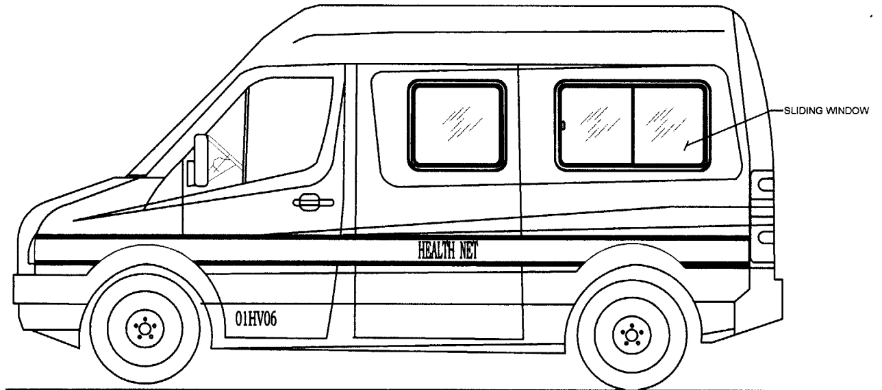
LHS ELEVATION
