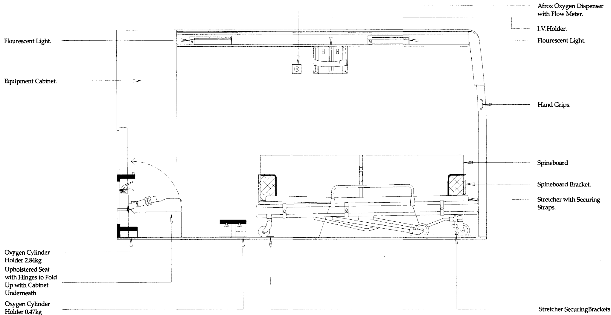
Right Inside Elevation
