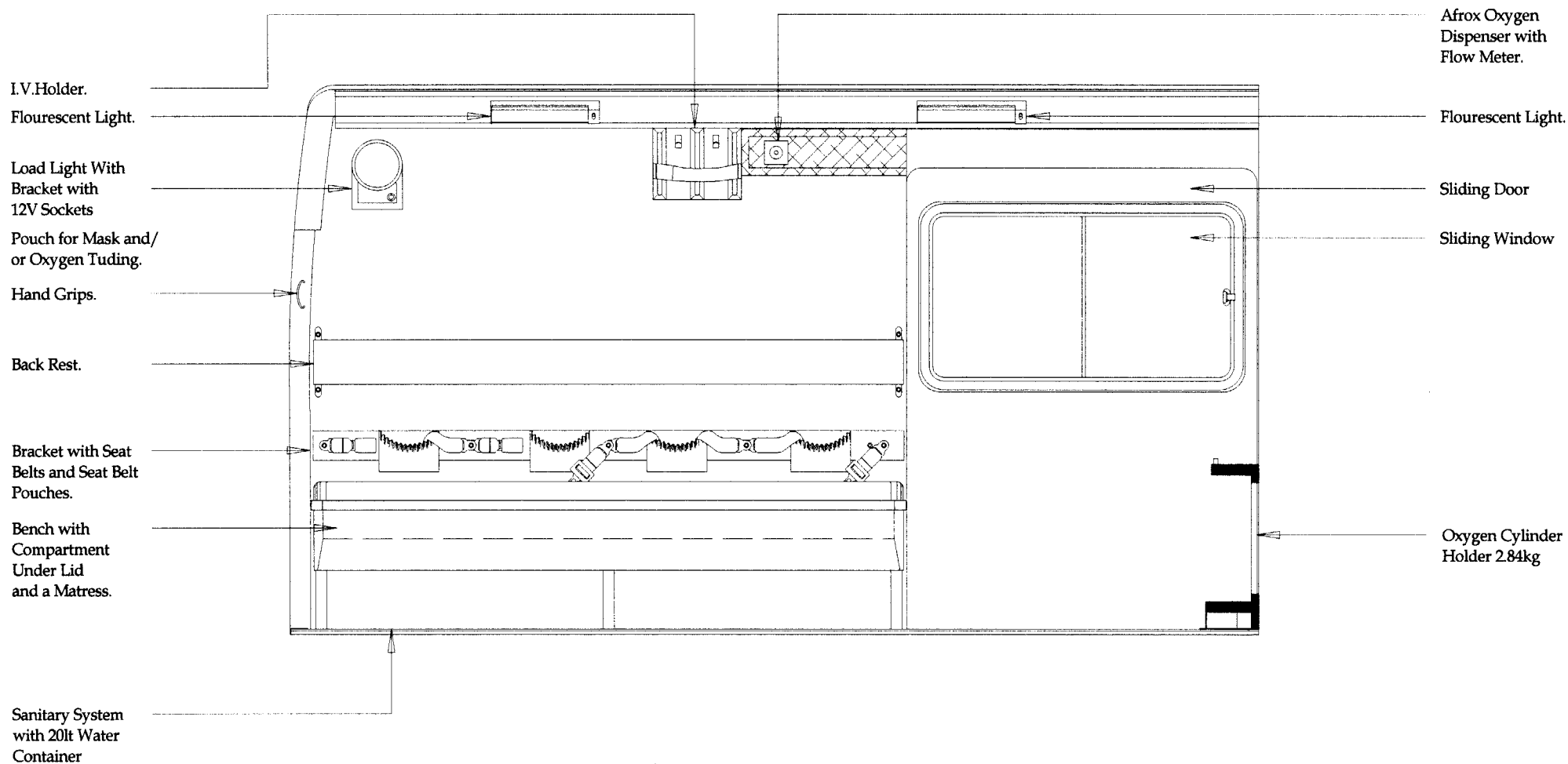
Left Inside Elevation
