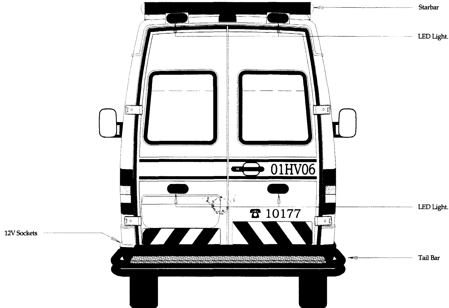
Back Outside Elevation
