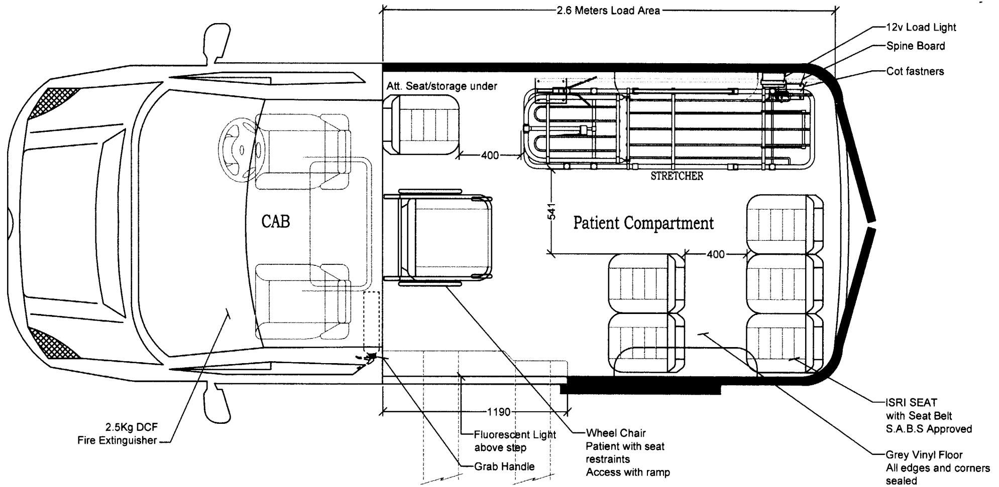
Plan View
