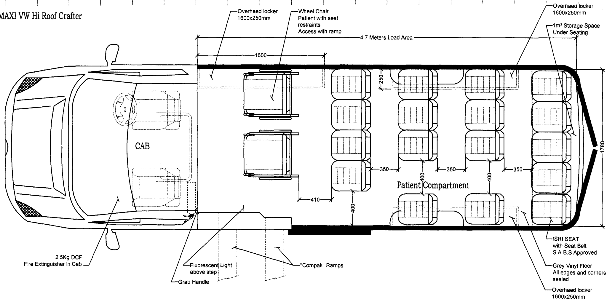
Plan View
