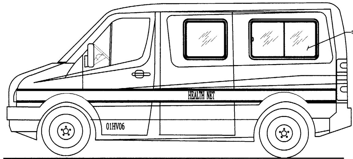
LHS ELEVATION
