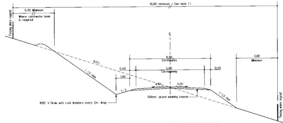
TYPE 7A LOCAL ROAD OR BY-ROAD (MOUNTAINOUS TERRAIN)
