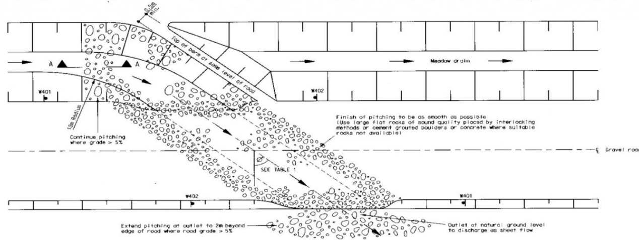
DISH CROSSING DETAIL
