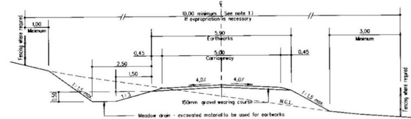
TYPE 7A LOCAL ROAD OR BY-ROAD (ROLLING TERRAIN)
