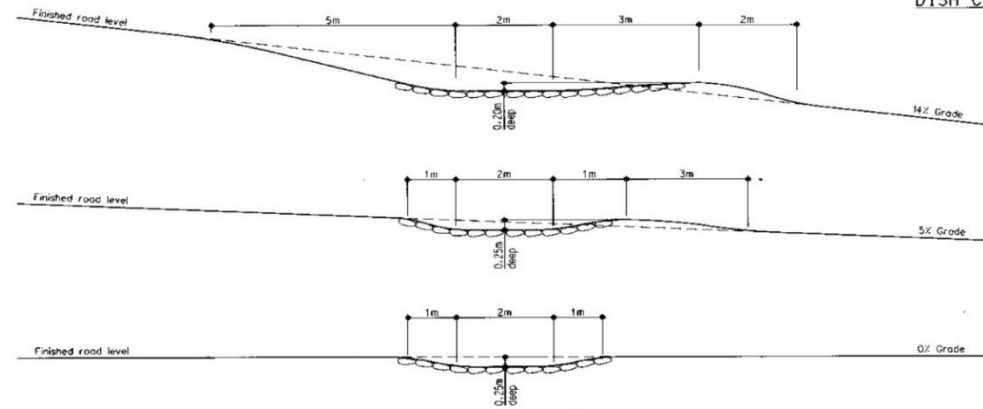
DISH CROSSING PROFILES
