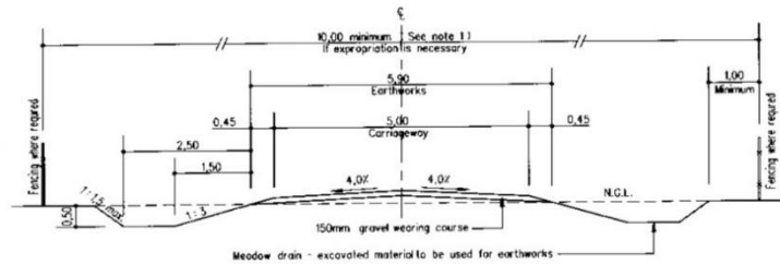
TYPE 7A LOCAL ROAD OR BY-ROAD (FLAT TERRAIN)
